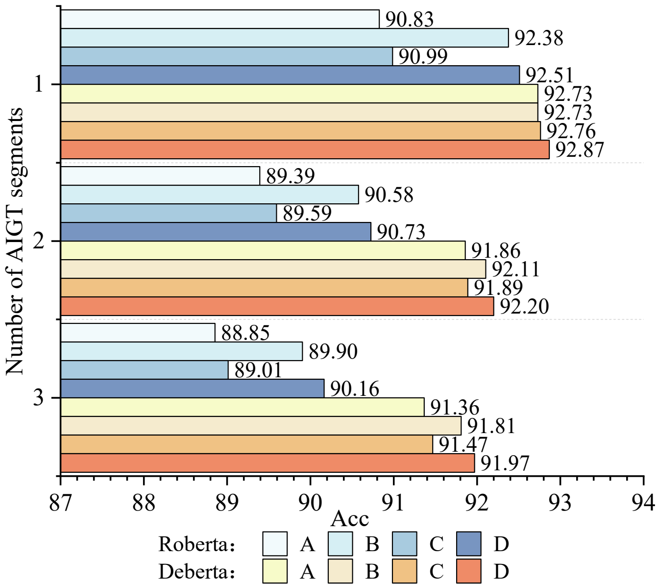
Acc based on GPT-2 generated text
